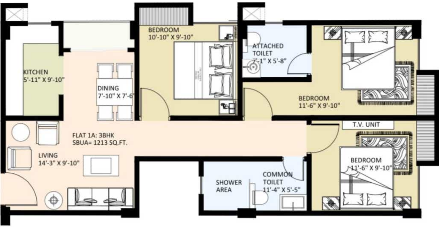
FIRST FLOOR
