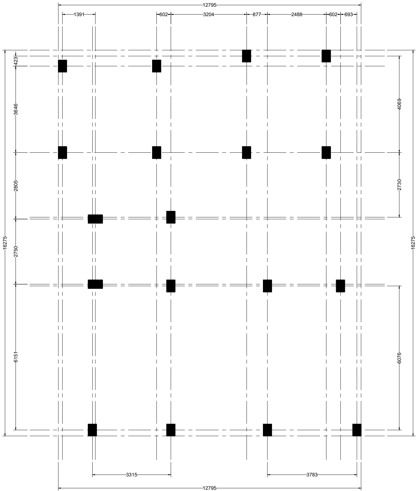
COLUMN LAYOUT
